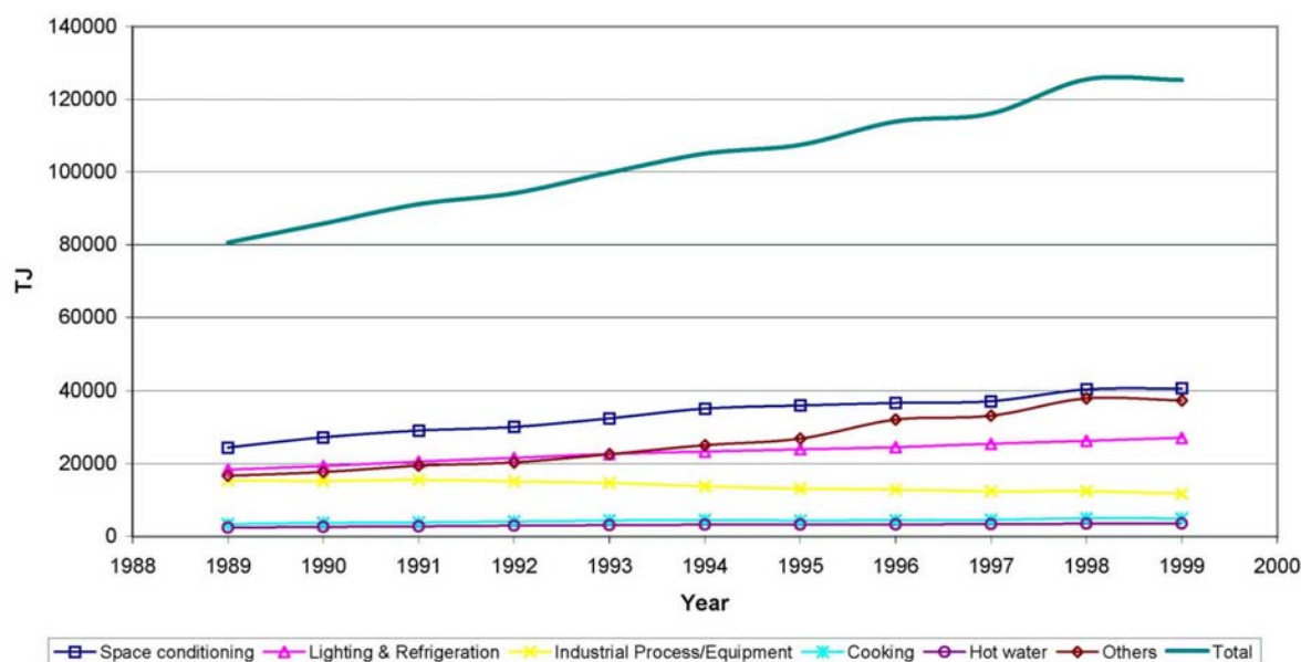
Figure 4-1: Electricity Consumption by End-use (1989 - 1999) (Source: Hong Kong Energy End-use Data, 1989 - 1999, EMSD)
