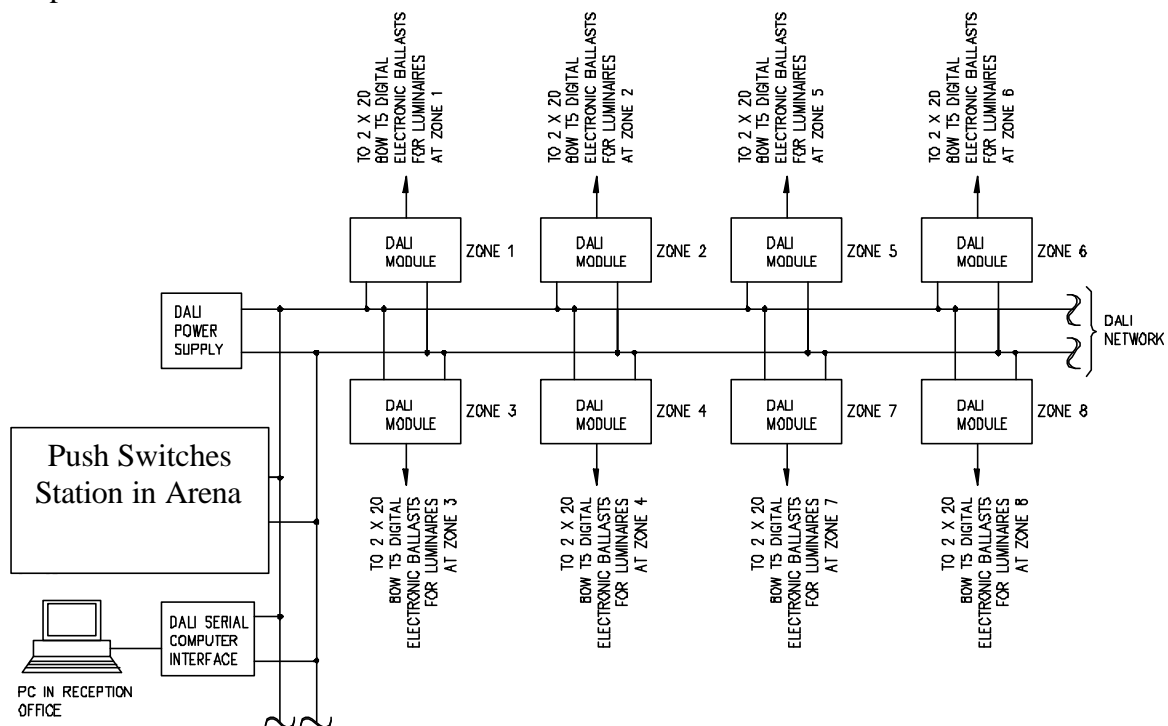
Fig. 7: DALI lighting control system for Kowloon Bay Indoor Games Hall
