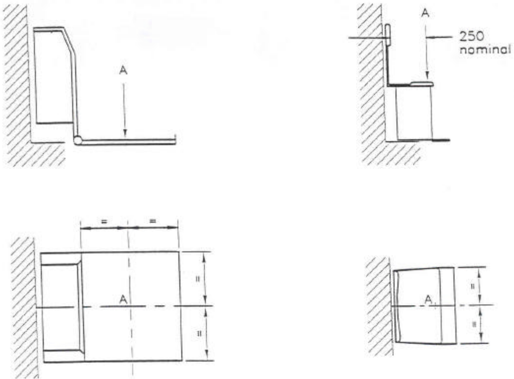
a) Wheel chair and standing passenger
