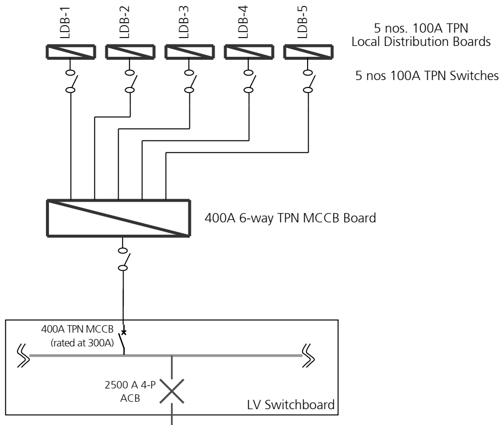
Figure 10.1.5.2 (a) : Schematic wiring diagram, existing
