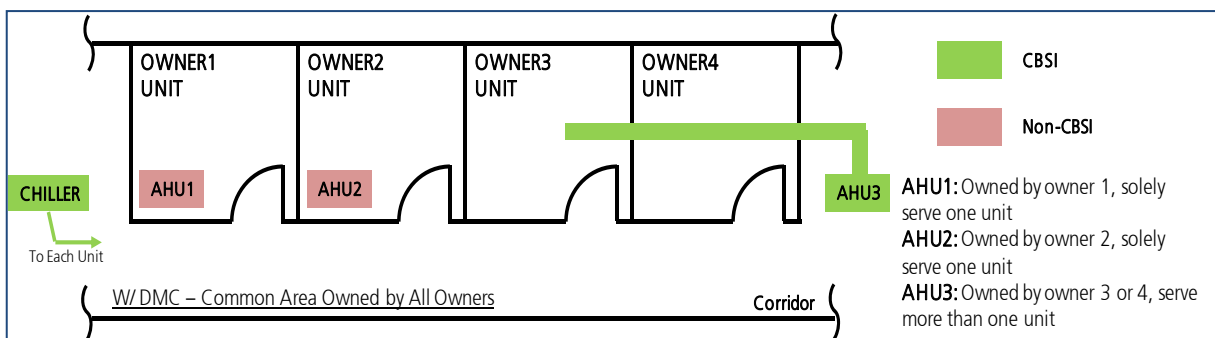
Figure 4.2.4 (a) : Diagram indicating examples of CBSI and non-CBSI for a Building with Common Area
