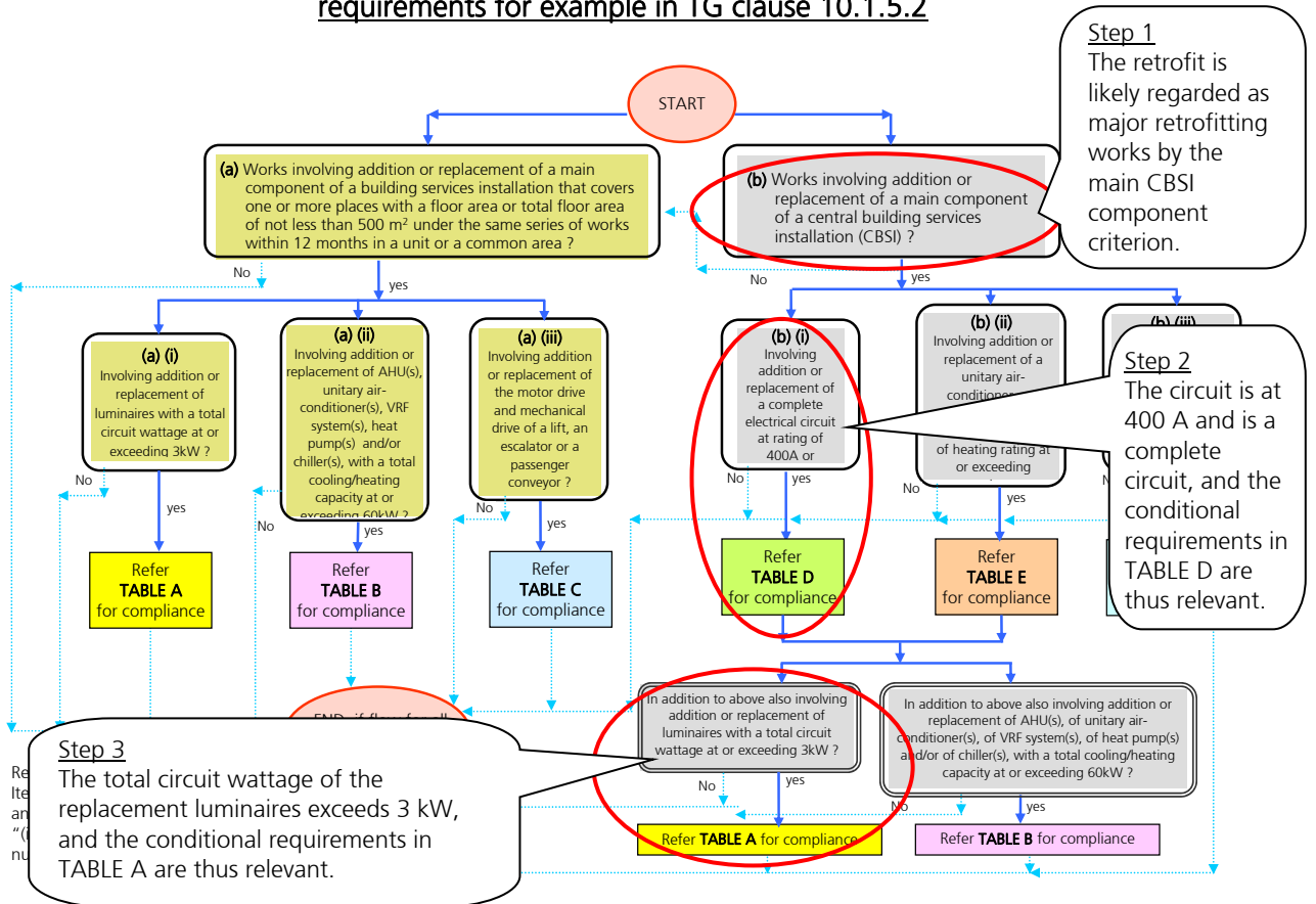
Figure 10.1.5.2 (c) : Illustration, against background of TG Figure 10.1, of energy efficiency requirements for example in TG clause 10.1.5.2
