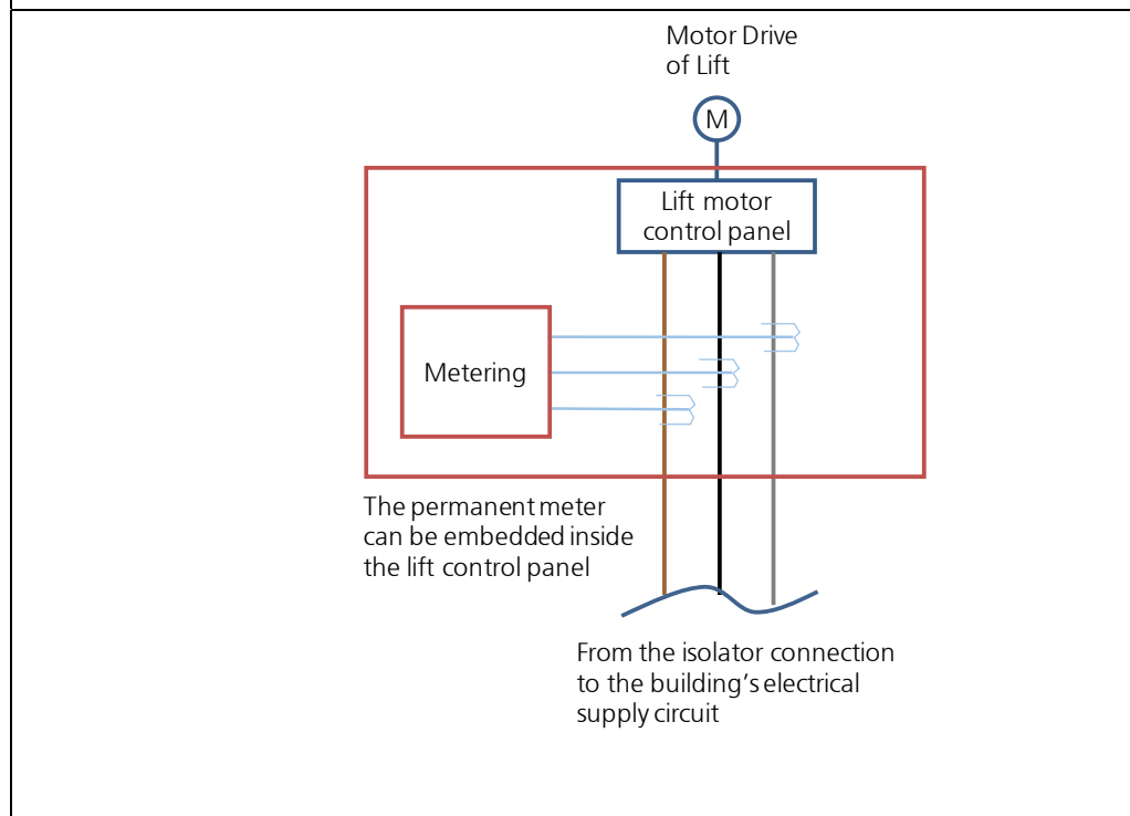
Figure 8.7 (a) : Illustrative diagram of provision of metering device for lift
