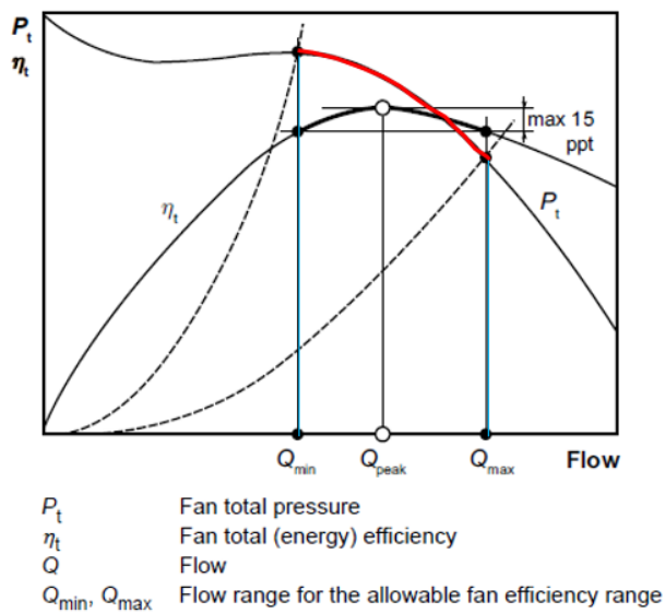
Figure 6.15 (c) : Allowable Selection Range within 15 percent point of Fan Peak Total Efficiency
