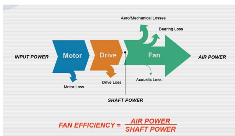
Figure 6.15 (a) : Fan Efficiency
