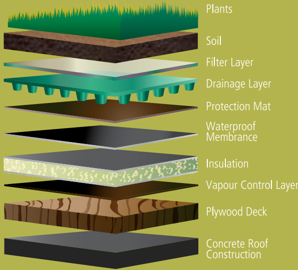
Typical Structure of an Extensive Green Roof
