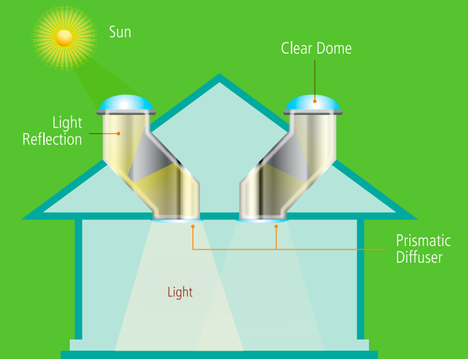
Working Principle of Light Tubes
