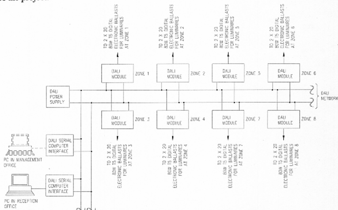
Fig. 13: Proposed DALI lighting control system for Kowloon Bay Indoor Games Hall
