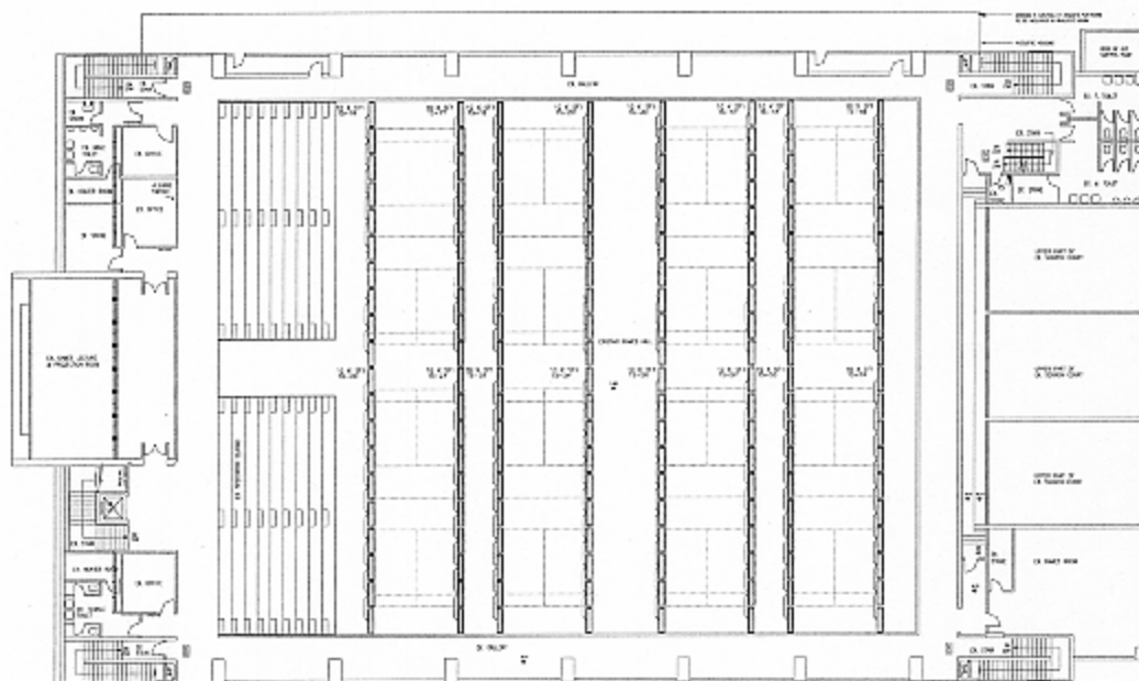
Fig. 12: Proposed lighting layout of the games hall using high output 80W T5 lamps
