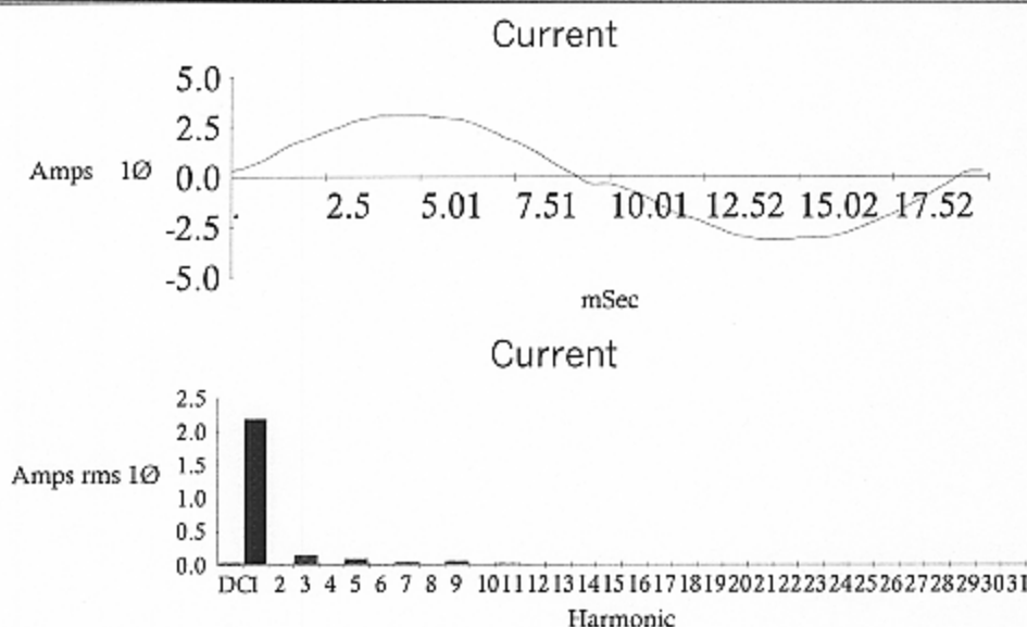
Fig.8: Current waveform and harmonic content of the new T5 luminaire
