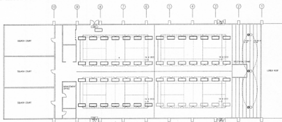
Fig. 4: Lighting layout of the new high output T5 lighting at EKT Indoor Games Hall
