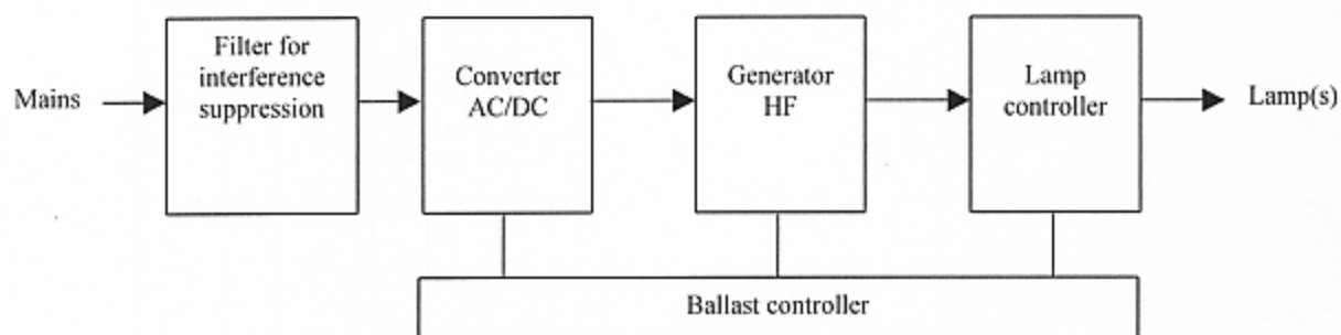
Fig. 1 Block diagram indicating main functions of electronic ballast
