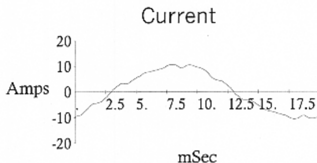
Fig. 8 Current waveform of the old 3x18W T8 luminaire
