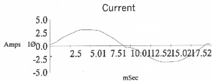
Fig. 9 Current waveform of the new T5 luminaire
