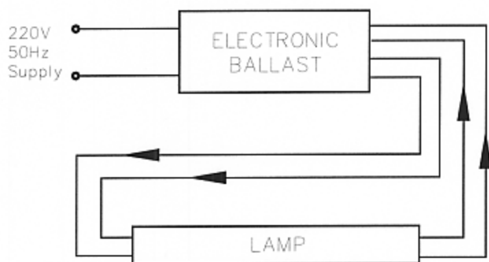
Fig. 2 Lamp circuit using electronic ballast
