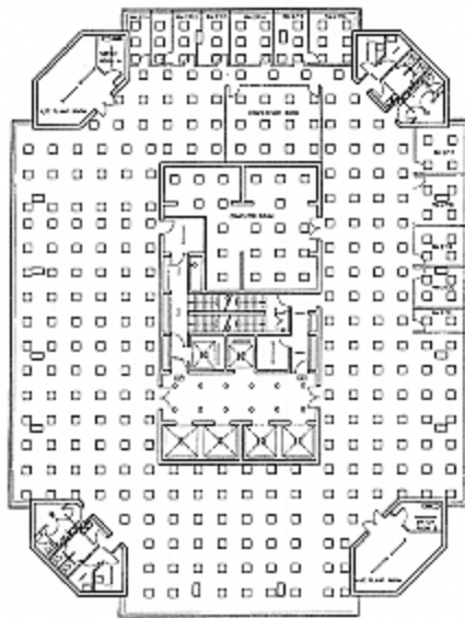
Fig. 6 Lighting layout at 27/F, Arsenal House
