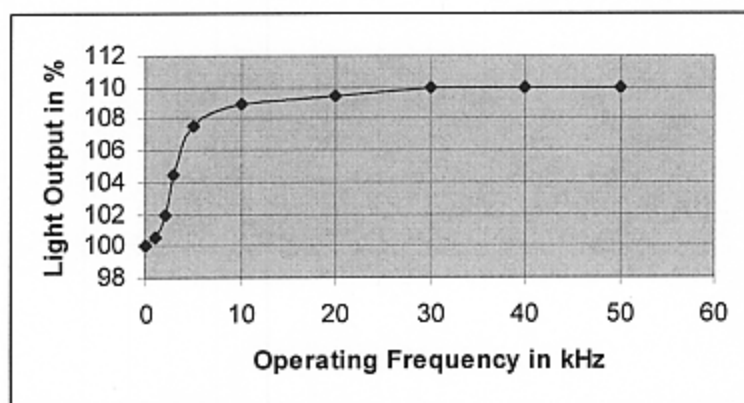
Fig. 3 Luminous flux of fluorescent lamp as a function of supply frequency at constant power
