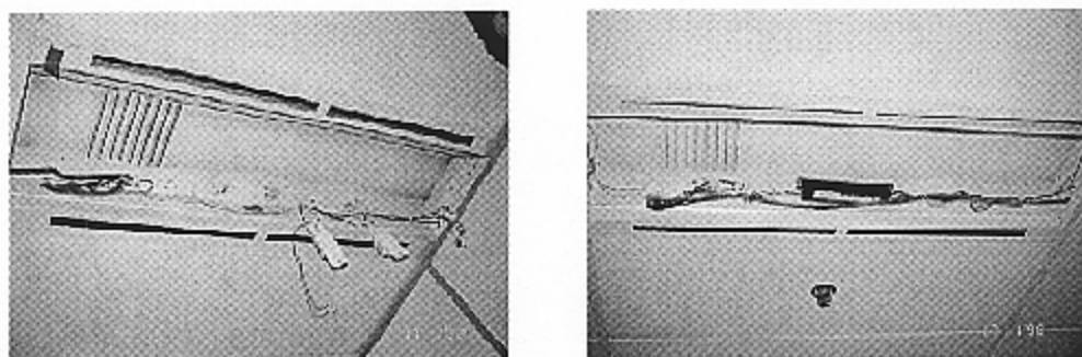
Fig. 5 Replacement of 2 nos. 36W Conventional Ballasts by 1 no. Electronic Ballast in Luminaire at Harbour Building
