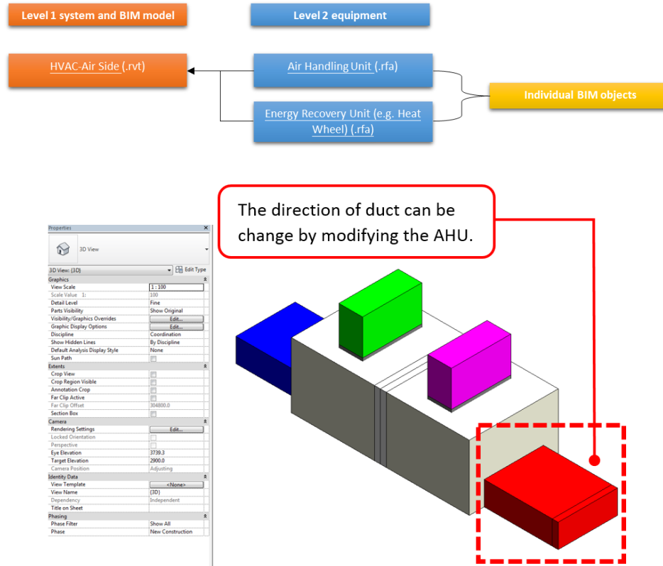
Figure 4-2 Object hierarchy for AHU
