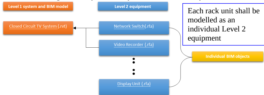
Figure 4-5 Object hierarchy for Close Circuit TV System
