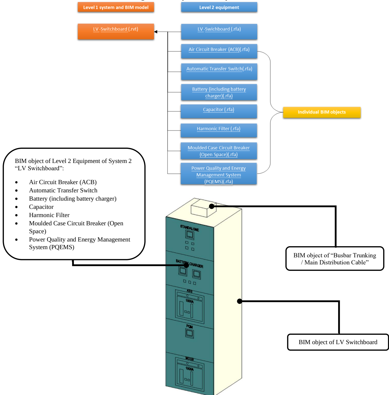
Figure 4-1 Object hierarchy for LV Switchboard
