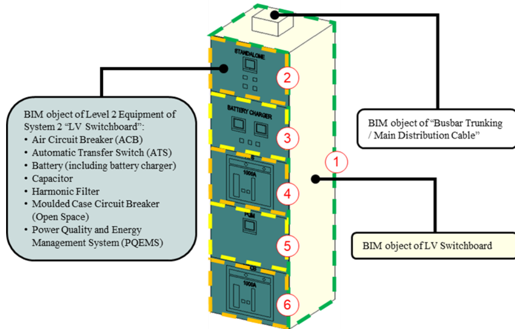
Figure 2-1 Example of nested object which is NOT applicable for LV switchboard installation
