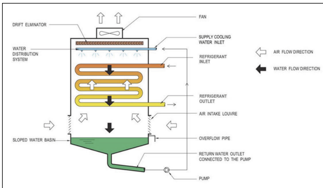
Figure 1.9: Typical configuration of evaporative condenser
