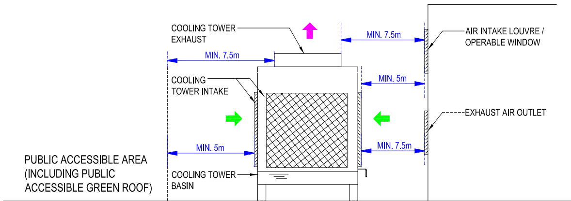
Figure B2 – Horizontal Separation
