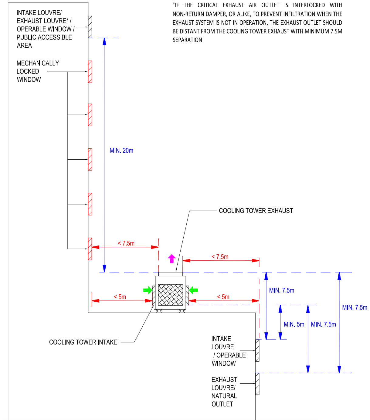
Figure B3 – Vertical Separation
