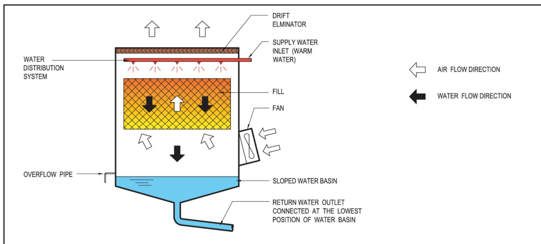
Figure 1.5: Typical configuration of forced draft counter flow cooling tower
