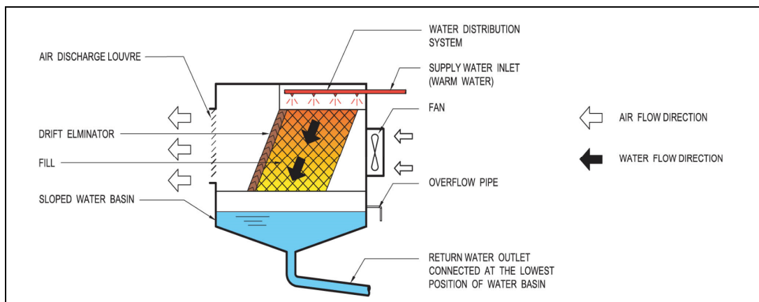
Figure 1.6: Typical configuration of forced draft cross flow cooling tower
