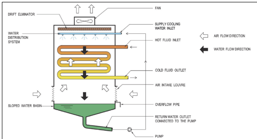
Figure 1.7: Typical configuration of closed-circuit cooling tower with no fill material
