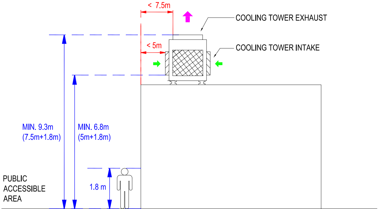
Figure B4 – Vertical Separation with public accessible area
