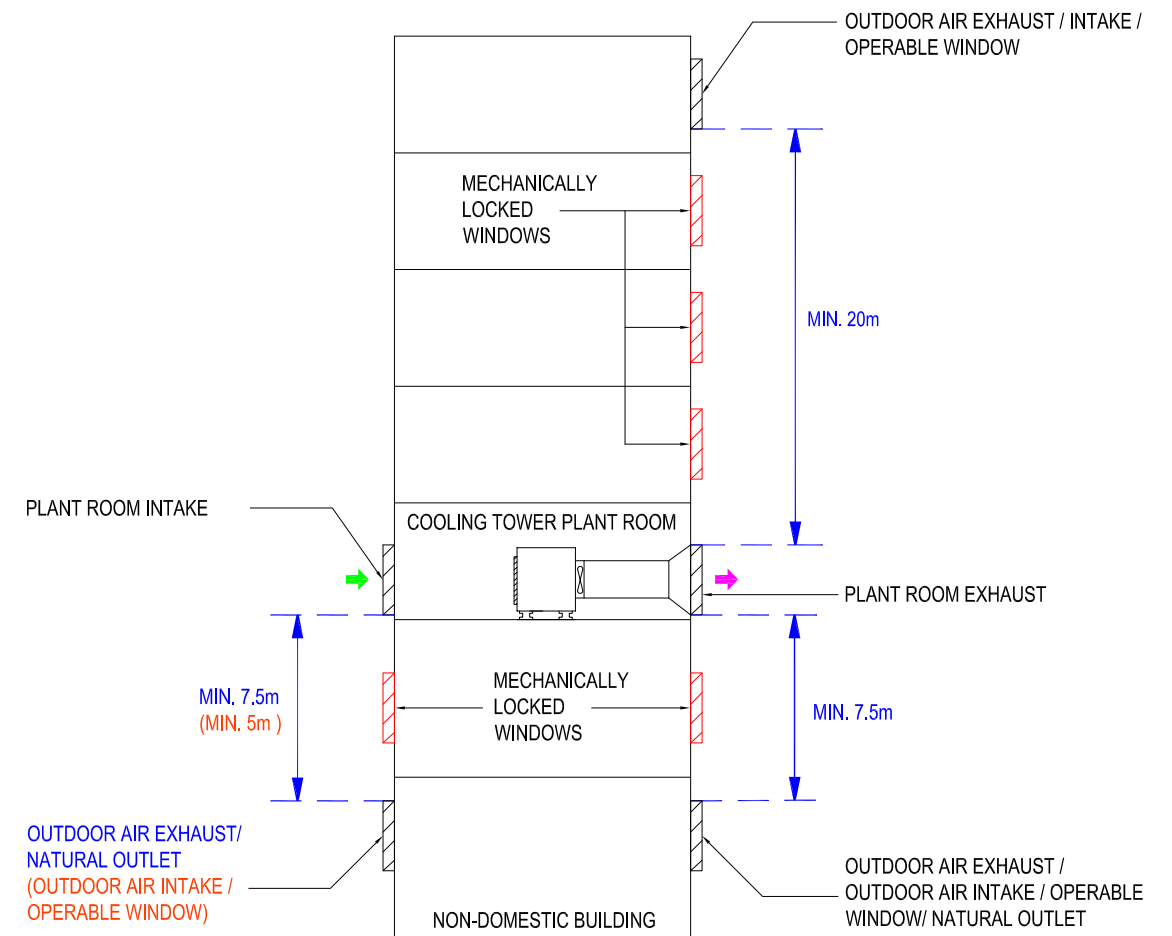
Figure B9 - Cooling tower at enclosed plant room
