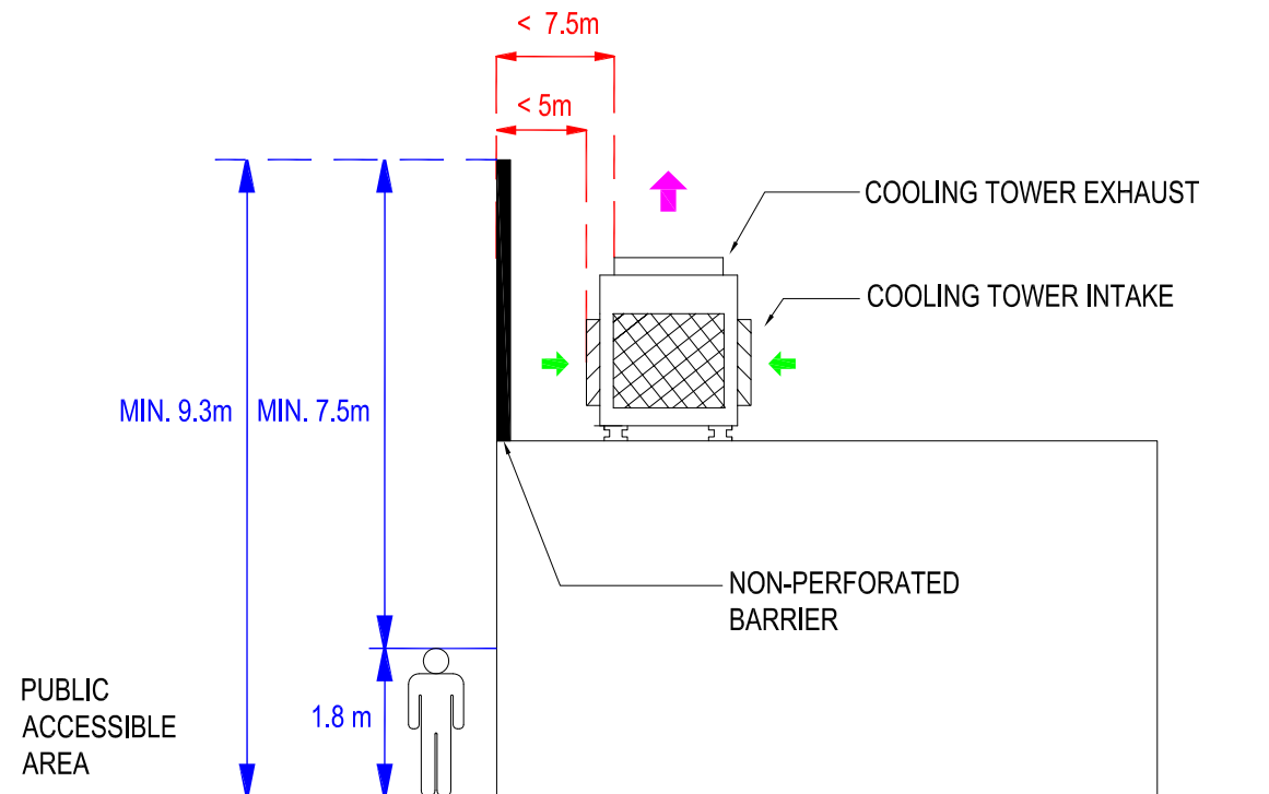
Figure B7 – Provision of non-perforated barrier
