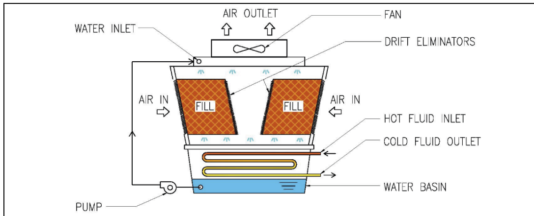
Figure 1.8: Typical configuration of coil shed cooling tower
