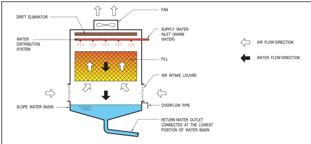
Figure 1.3: Typical configuration of induced draft counter flow cooling tower
