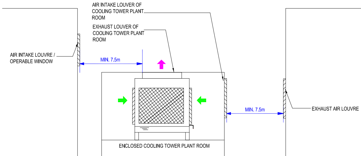
Figure B8 – Cooling tower at enclosed plant room
