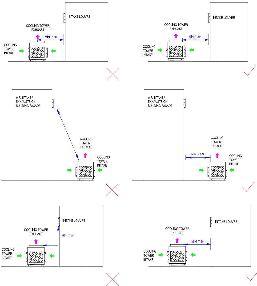
Figure B1 – General Separation Measurement
