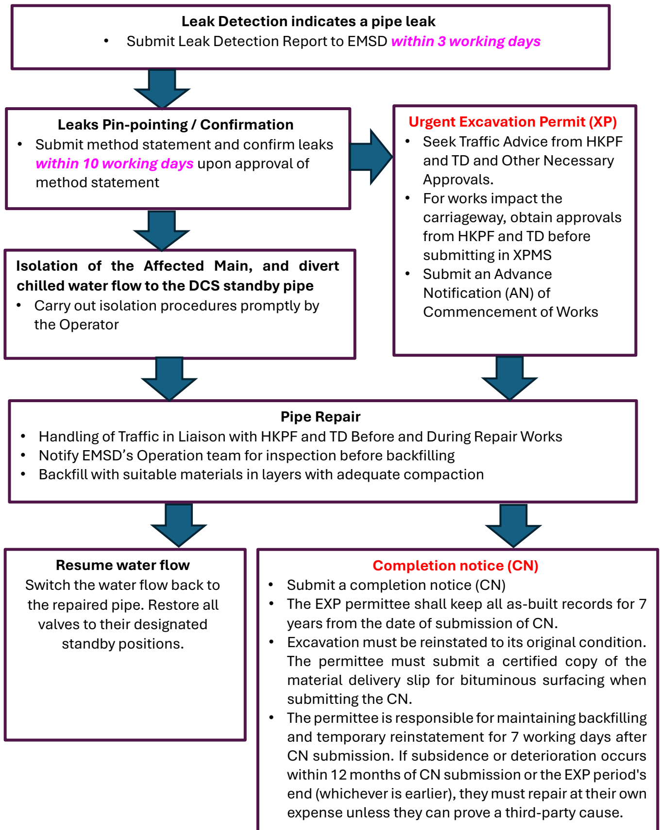
Figure 1: Workflow to repair pipe leaks
