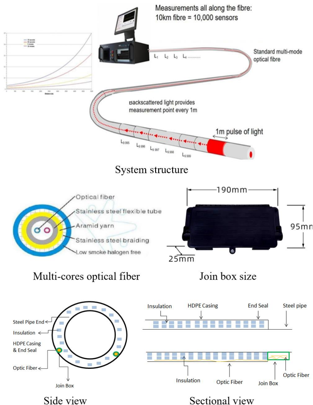
Figure 5: System structure of distributed fibre optic sensing technology for pipeline health monitoring
