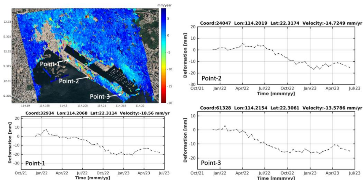
Figure 9: An example dashboard for real-time monitoring of pipe settlement (with reference of Kai Tak DCS)
