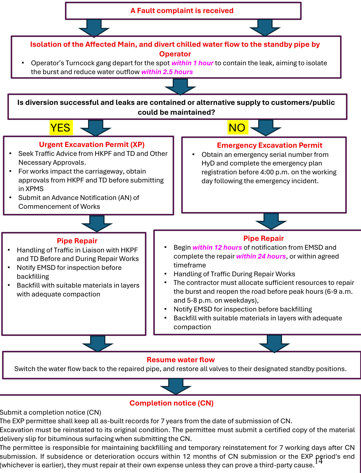
Figure 2: Workflow to repair pipe bursts
