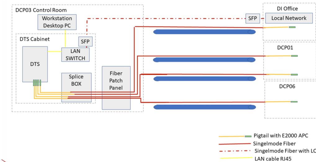
Figure 4: Example DTS System Architecture
