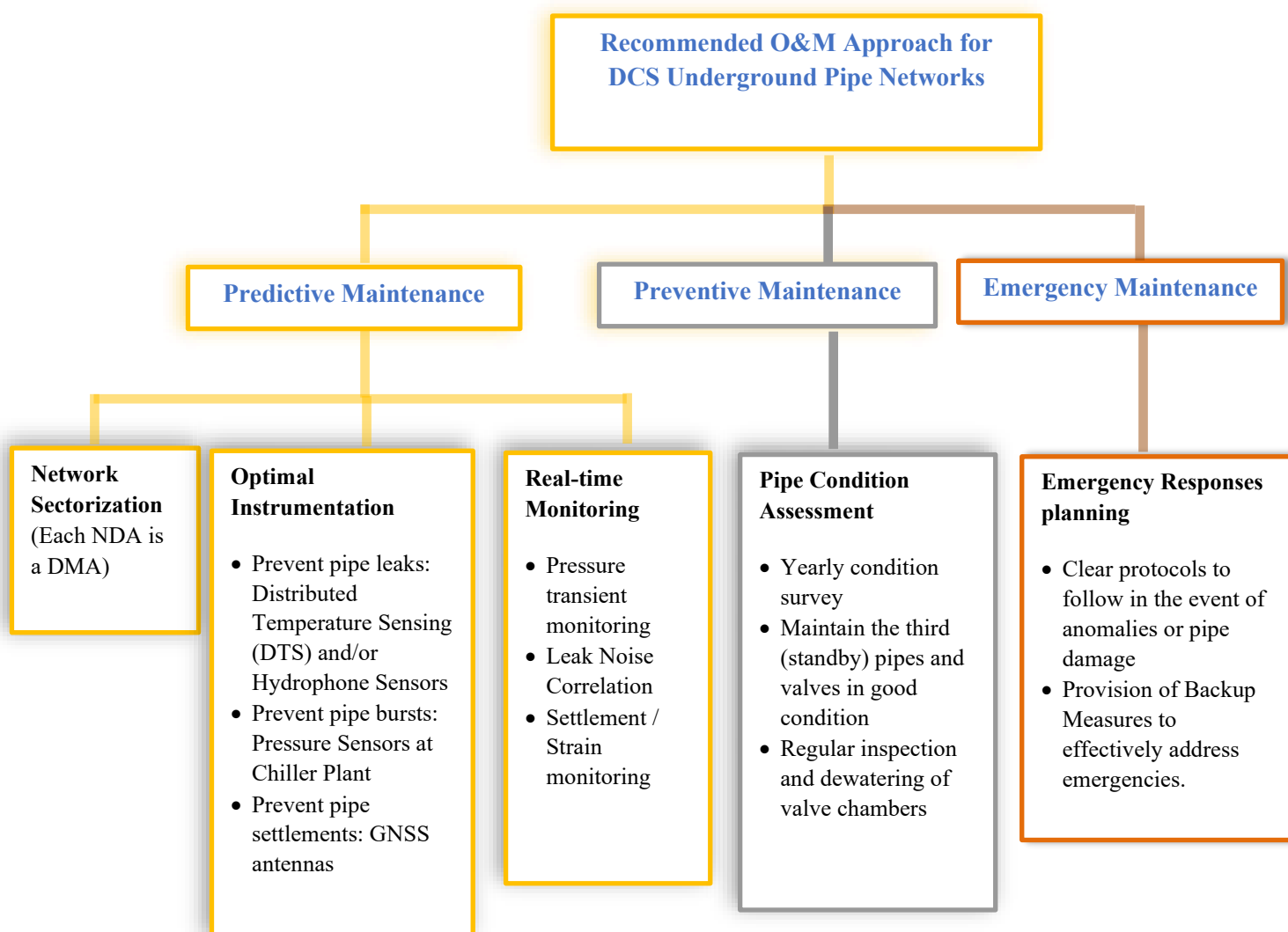
Figure 1: O&M Approach for DCS Underground Pipe Networks
