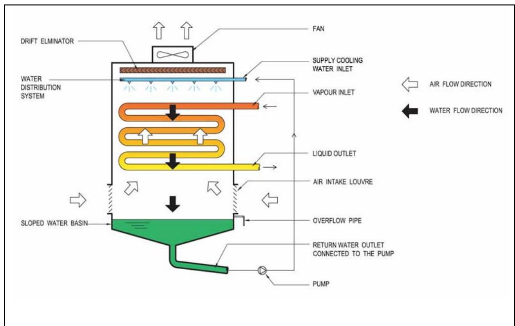
Figure 1.8: Typical configuration of evaporative condenser
