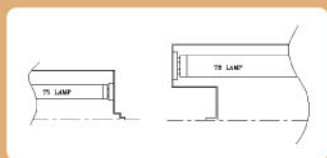
Figure 11 - Recessed 50mm modular T5 luminaire (left) and 100mm T8 luminaire with extruded endbox (right)
