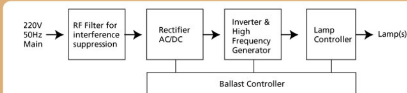
Figure 3 - Block diagram indicating main functions of electronic ballast
