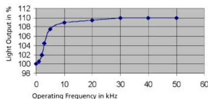
Figure 4 - Luminous flux of fluorescent lamp as a function of operating frequency
