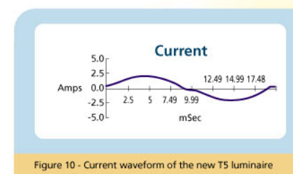
Figure 10 - Current waveform of the new T5 luminaire
