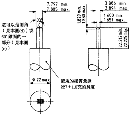
(a) 接地插座觸點規
