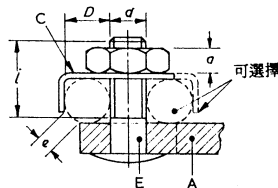
螺柱式終端
