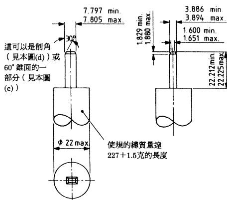
(a) 接地插座觸點規
