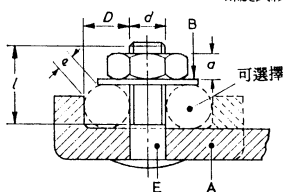
螺柱式終端
