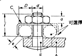
螺柱式終端
